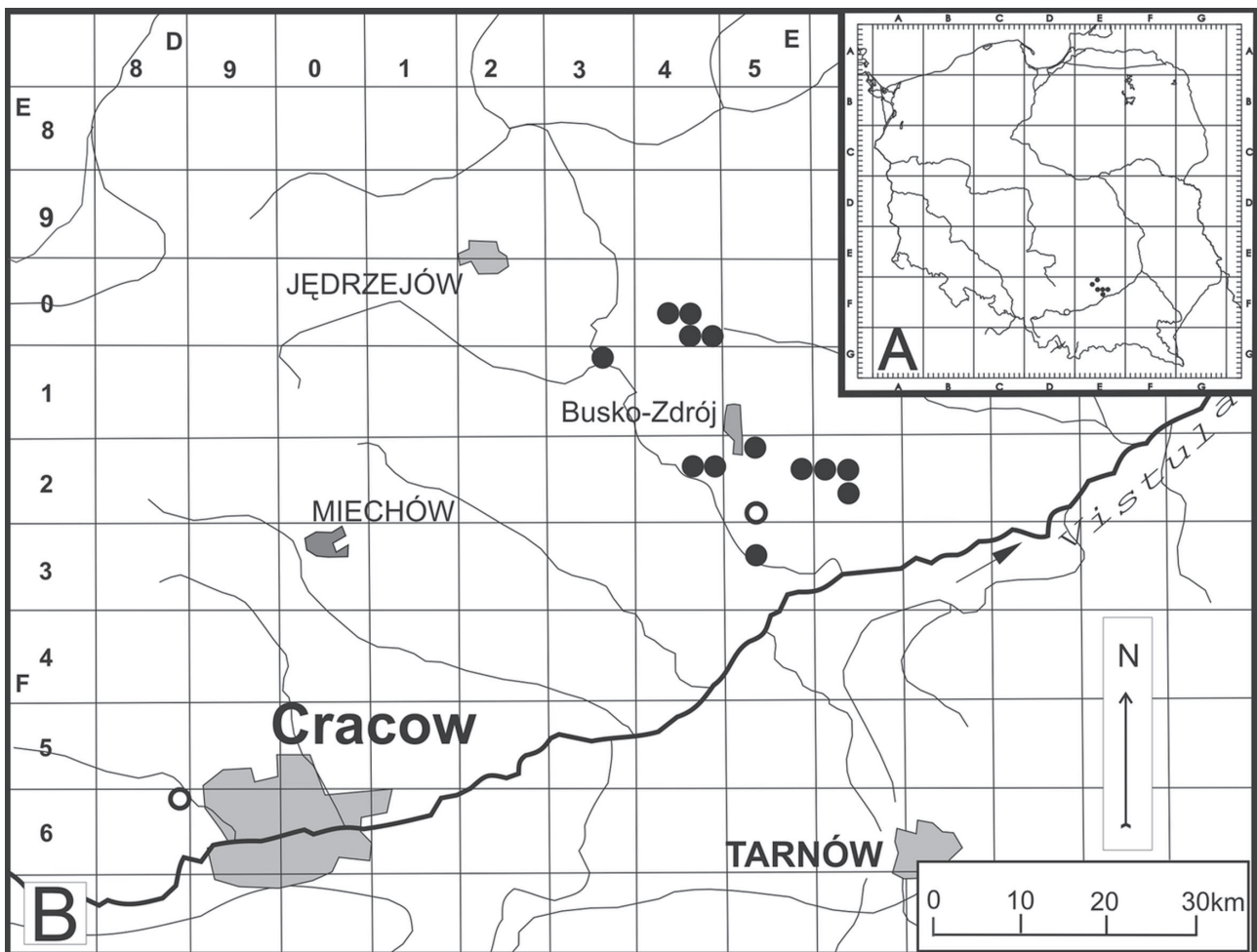
Fig. 1. Distribution maps of Arabis recta Vill. Explanations A – in Poland (in the ATPOL grid of squares 10 km x 10 km), B – in the Małopolska Upland (in the ATPOL grid of squares 2.5 km x 2.5 km), ● – locality existing at present, ○ – locality not confirmed
